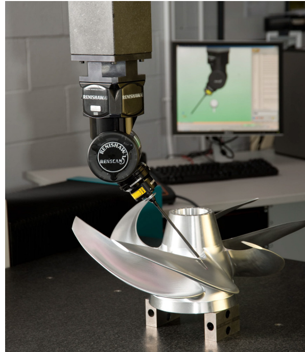
Reniscan5 allows TURBOCAM to do continuous, automated measurement of complex turbomachinery components, collecting thousands of points to verify form
